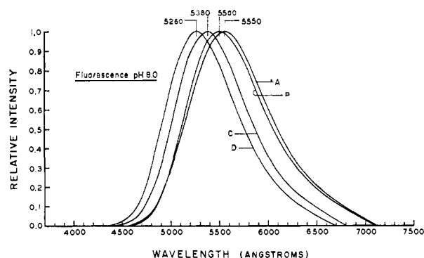
Figure 4. Fluorescence emission spectra of (A) dehydroluciferin (VI), (B) 4'-hydroxyluciferin (V), (C) luciferin (I), (D) aminoluciferin (IVa) in glycylglycine buffer at pH 8.0. Spectra are normalized to 1 at peak emission.
