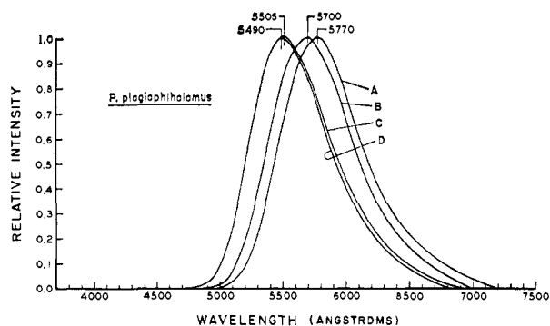
Figure 3. In vitro bioluminescence emission spectra of (A) P. plagiophthalmus ventral organ luciferase plus luciferin (I), (B) P. platiophthalmus ventral organ luciferase plus aminoluciferin (IVa), (C) P. platiophthalmus dorsal organ luciferase plus luciferin (I), (D) P. plagiophthalmus dorsal organ luciferase plus aminoluciferin (IVa). All reactions run in 0.025 M glycylglycine buffer at pH 7.6. The spectra are normalized to 1 at peak emission.
